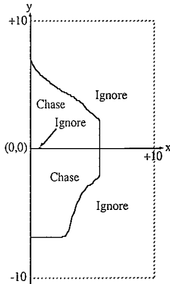
Figure 10 Switching curve of the best-of-generation program from generation 25 for version 1.
