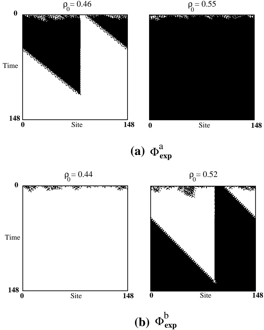
Figure 5: Space-time behavior of two “block expanding” CAs evolved on different GA runs. (a) \phi_{exp}^a with \rho_0 = 0.46 (left) and \rho_0 = 0.55 (right). This CA defaults to a fixed point of all 1s unless the IC contains a sufficiently large block of adjacent 0s, in which case, that block is expanded. (b) \phi_{exp}^b with \rho_0 = 0.44 (left) and \rho_0 = 0.52 (right). This CA defaults to a fixed point of all 0s unless the IC contains a sufficiently large block of adjacent 1s, in which case, that block is expanded. The classification of the IC is correct in each of these four cases.
