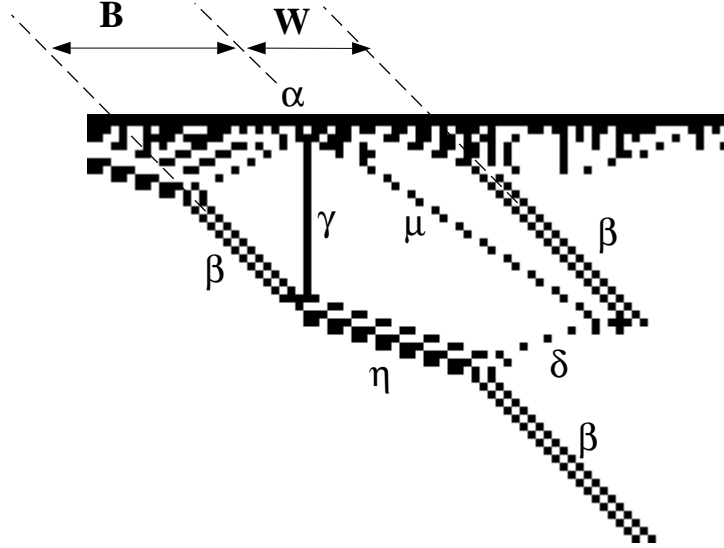
Figure 12: Blow-up of part of right-hand diagram of Fig. 8b, illustrating asymmetries in \phi_{\text{par}}^{\text{b}} 's particle velocities that can result in misclassifications.
