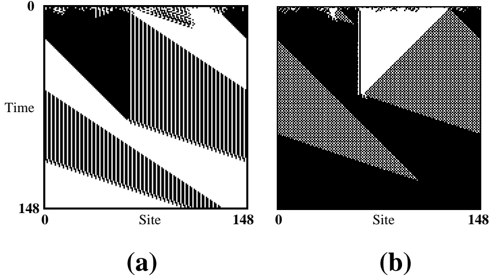
Figure 11: (a) Misclassification by \phi_{\text{par}}^{\text{b}} , with \rho_0 = 0.52 . (By T_{\text{max}} = 2N , the CA reaches an all-0s fixed point.) (b) Correct classification by \phi_{\text{par}}^{\text{a}} on the same IC.
