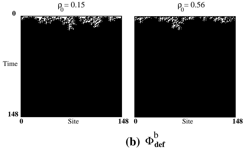
Figure 4: Space-time behavior of “default” strategy CAs evolved on two different GA runs. (a) \phi_{\text{def}}^a with \rho_0 = 0.48 (left) and \rho_0 = 0.74 (right). On almost all ICs this CA iterates to a fixed point of all 0s, correctly classifying only low- \rho ICs. (b) \phi_{\text{def}}^b with \rho_0 = 0.15 (left) and \rho_0 = 0.56 (right). On almost all ICs this CA iterates to a fixed point of all 1s, correctly classifying only high- \rho ICs.
