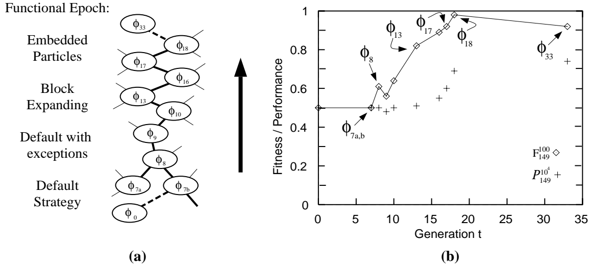
Figure 13: (a) Partial ancestral tree of \phi_{\text{par}}^{\text{a}} . (b) F_{149}^{100}(\phi) (diamonds) and \mathcal{P}_{149}^{10^4}(\phi) (crosses) of the CAs \phi_i in (a). Six of the data points are marked with the name of the corresponding CA.
