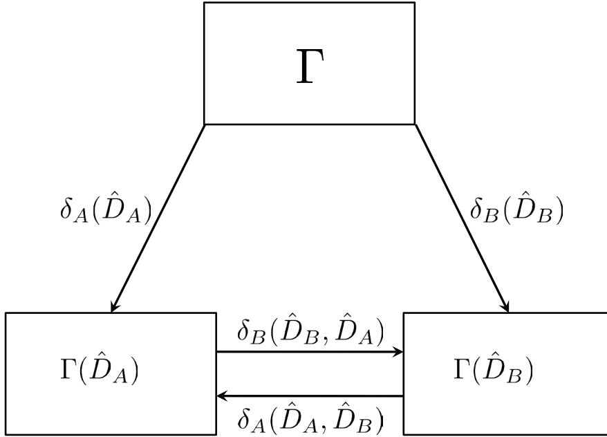
Fig. 1 This diagram depicts a flow between \Gamma , \Gamma(\hat{D}_A) and \Gamma(\hat{D}_B) based on the willingness to pay of players A and B .
