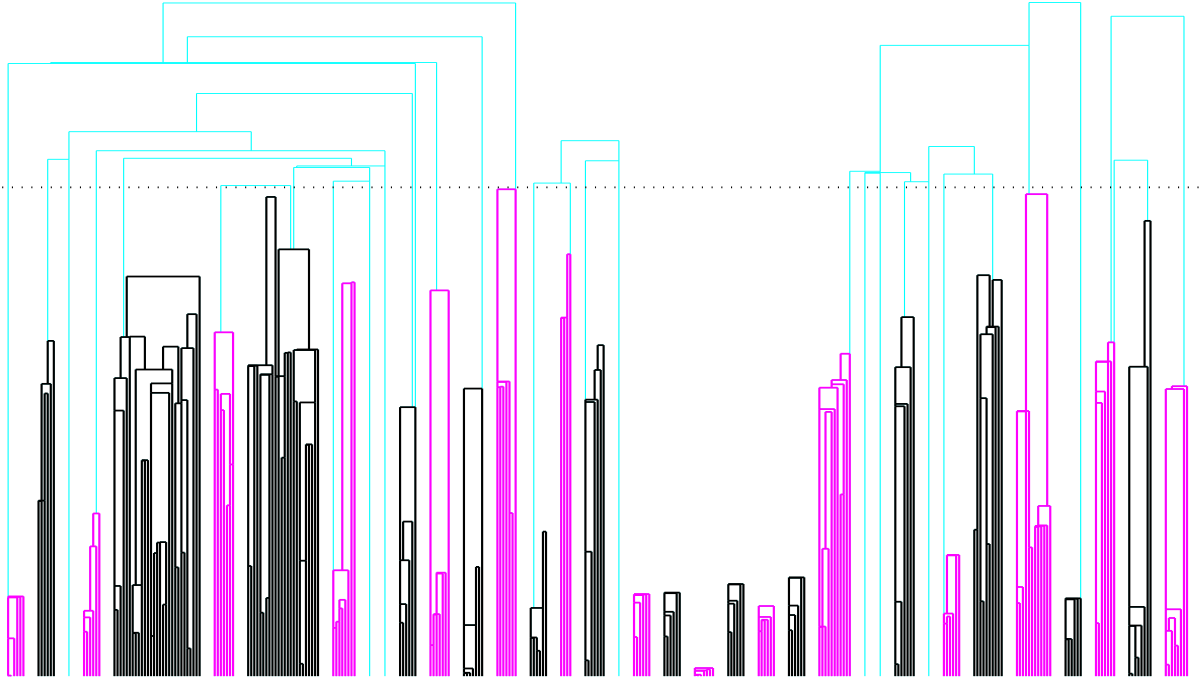
FIG. 2. The hierarchical tree or dendrogram showing community structure for a network with N = 250 , \kappa = 0.01 , \beta = 5 , calculated as described in the text. In this case, we have designated separate communities by whether their lowest connecting path in the tree falls above or below a specified threshold, indicated by the horizontal dotted line, and the components have been spaced out and colored to illustrate this designation. The threshold value is chosen using a criterion based on the density of edges within components as described in Ref. [26].
