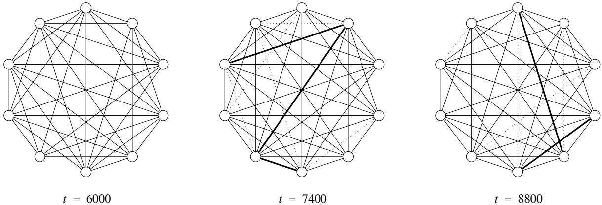
FIG. 5. Time evolution of the edges within one component for \beta = 1.25 and \kappa = 0.01 . Dotted lines indicate connections that existed in the previous frame and have since decayed. Bold lines indicate new connections. All new connections are made with vertices already included in this group.
