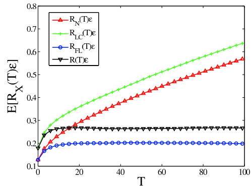
FIG. 3: A comparison of cumulative price impacts when different effects are included. R_N(T) (red up triangles) is the naive cumulative price impact calculated as a sum of fixed price impacts with no liquidity variation and no variable quote updating. R_{LC}(T) (green crosses) includes the effect of non-transaction driven quote changes but does not include fluctuating liquidity. R_{FL}(T) (blue circles) includes the effect of the liquidity imbalance, without including any effect of non-transaction driven quote changes. Finally, R(T) (black down triangles) corresponds to the real cumulative price impact. All results are for the stock Vodafone Group based on the on-book data from 2000 – 2002. Returns are in units of the average spread, which is approximately 0.00246 in logarithmic price.
