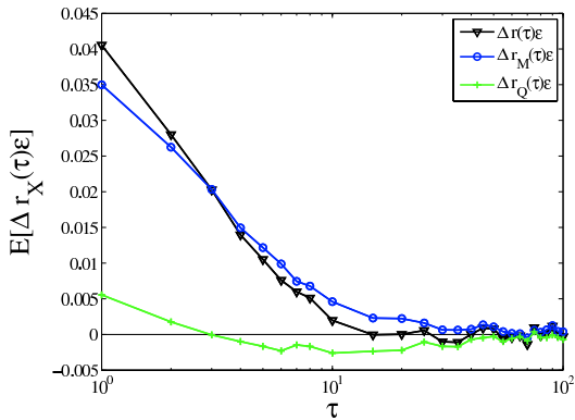
FIG. 2: A comparison of \Delta r(\tau) (black down triangles), \Delta r_M(\tau) (blue circles) and \Delta r_Q(\tau) (green crosses) for the stock AstraZeneca based on on-book data from 2000 – 2002. Returns are in units of the average spread, which is 0.00154 in logarithmic price.
