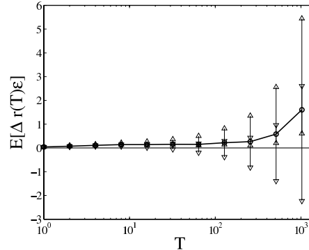
FIG. 4: A crude estimate of the statistical errors in the price impact at different times for Astrazeneca based on the on-book data for 2000-2002 based on equation 4 (triangle up). The circles are the estimated mean impact. For comparison the figure shows also standard errors (triangle down). Returns are shown in units of the average spread.
