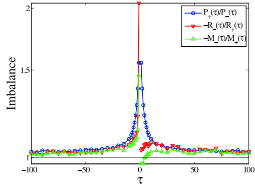
FIG. 1: A comparison of the transaction imbalance P_+(\tau)/P_-(\tau) (blue circles), return imbalance -R_-/R_+ (red down triangles), and liquidity imbalance -M_-(\tau)/M_+(\tau) (green up triangles), for the stock Astrazeneca based on on-book data from 2000–2002. Note that we have excluded values at \tau = 0 , where they diverge or are undefined; the peaks occur at \tau = -1 .
